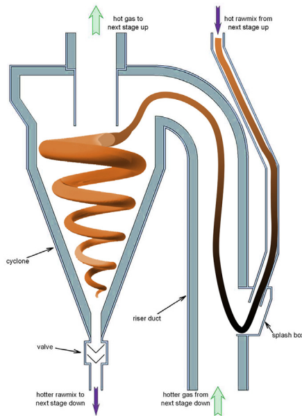
1 The residual exhaust of alternative fuels can abet accumulations and blockages throughout in the preheater
